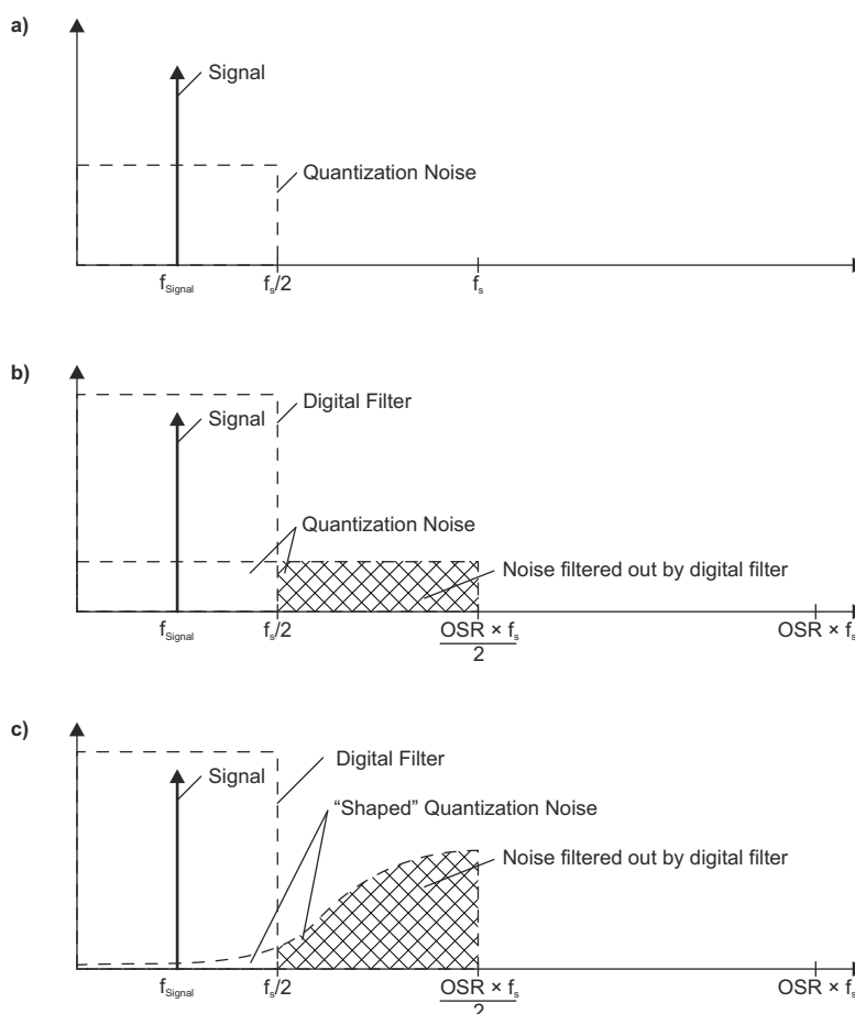
Figure 13-2. Sigma-Delta Principle
