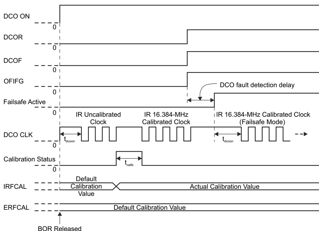
Figure 4-4. DCO Operation With External Resistor – Fault at Startup
