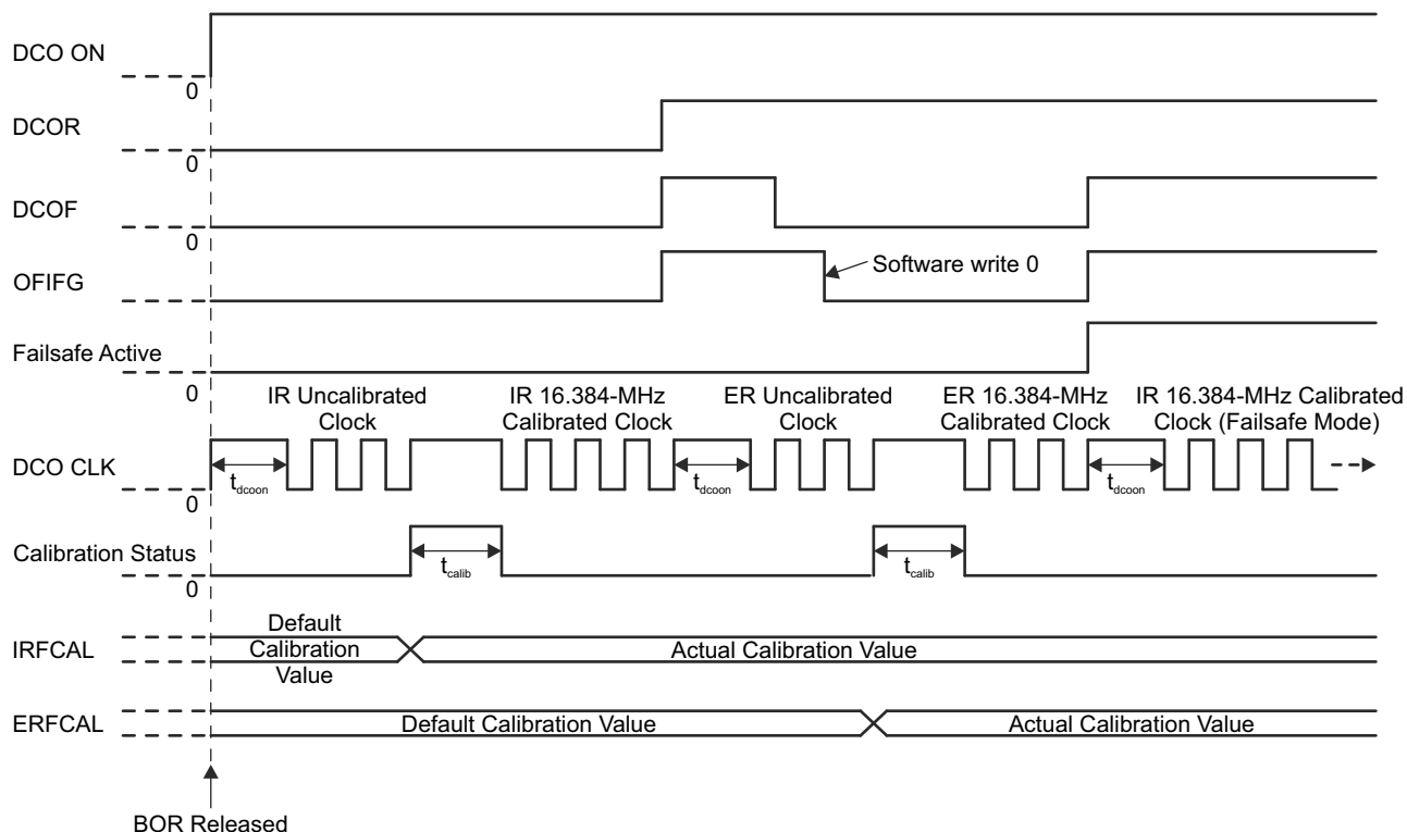
Figure 4-5. DCO Operation With External Resistor – Fault During Run Time
