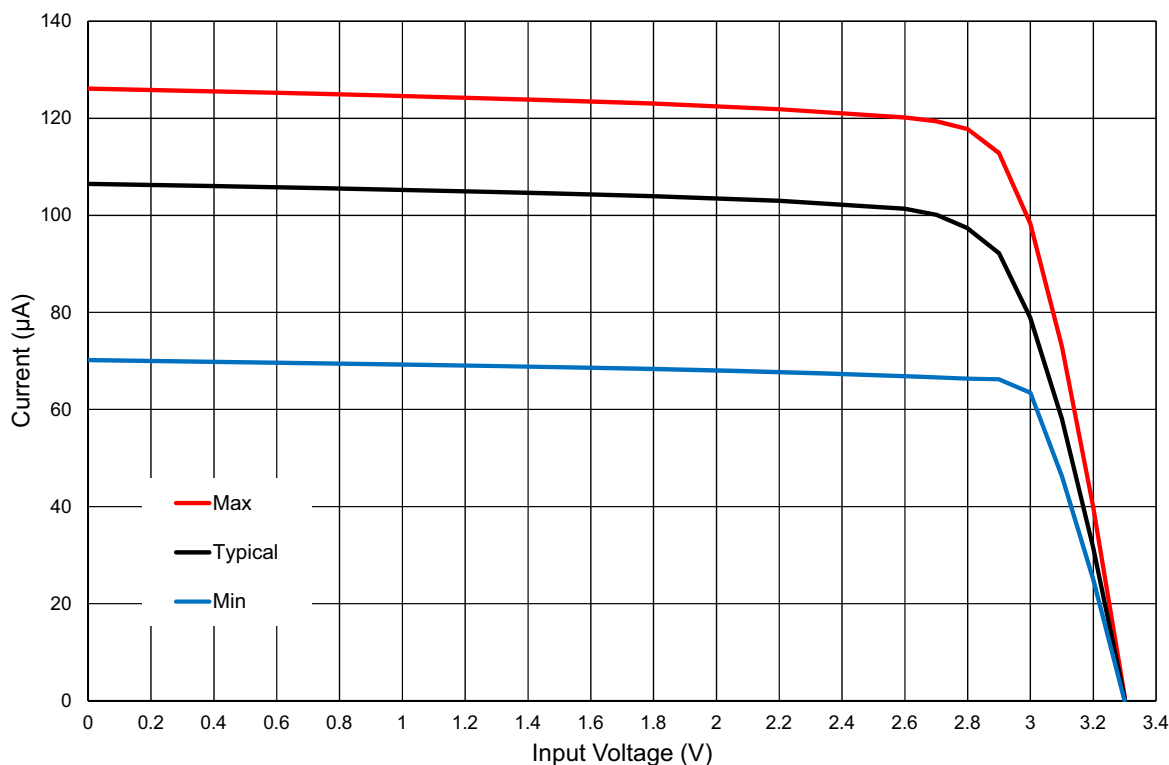
Figure 66: ACMP Input Current Source vs. Input Voltage at T = -40 °C to 105 °C, VDD = 3.3 V
