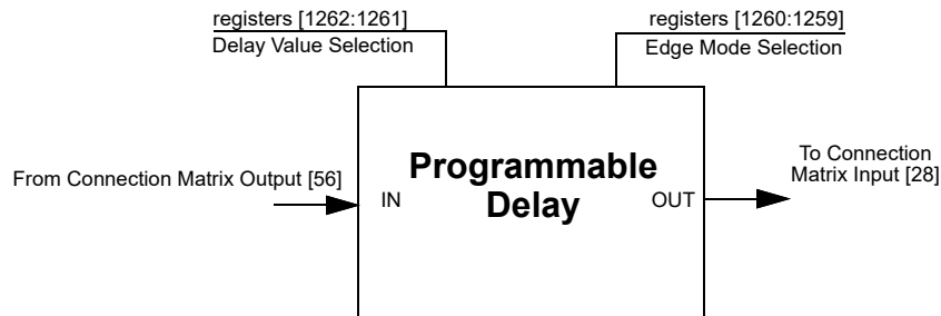
Figure 67: Programmable Delay
