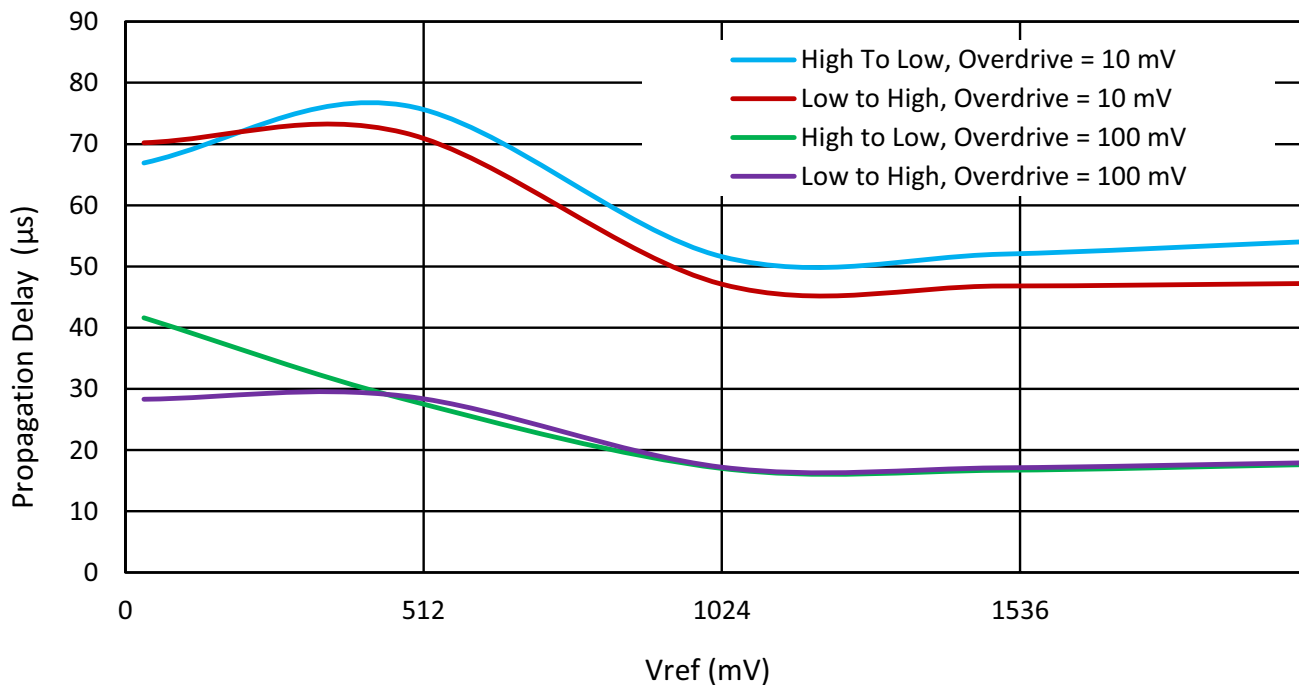
Figure 60: Typical Propagation Delay vs. V_{\text{ref}} for ACMPxL at T = 25\text{ }^{\circ}\text{C} , Gain = 1, Buffer - Disabled, Hysteresis = 0
