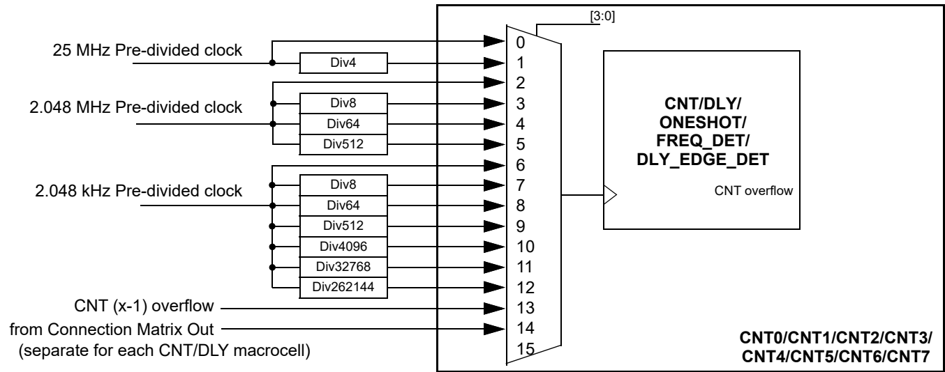
Figure 78: Clock Scheme
