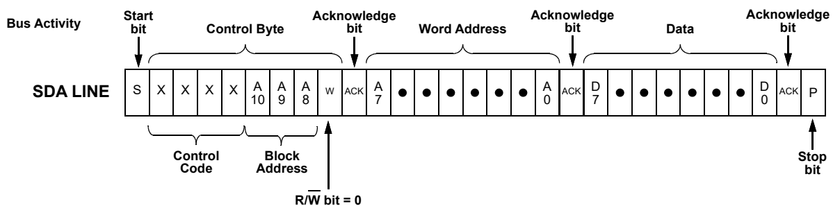
Figure 92: Byte Write Command, \overline{R/W} = 0
