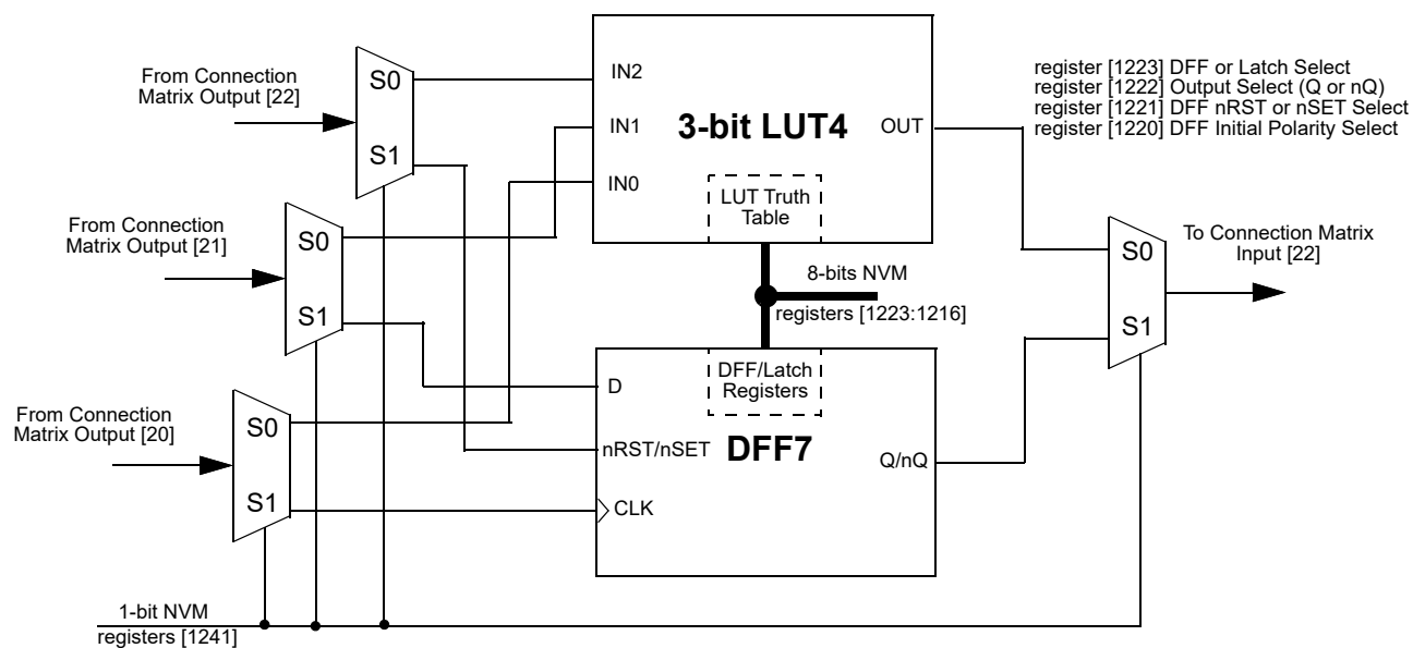
Figure 22: 3-bit LUT4 or DFF7
