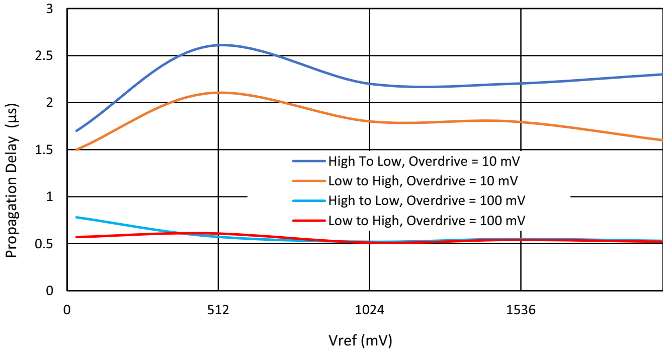
Figure 59: Typical Propagation Delay vs. V_{\text{ref}} for ACMPxH at T = 25\text{ }^{\circ}\text{C} , Gain = 1, Buffer - Disabled, Hysteresis = 0
