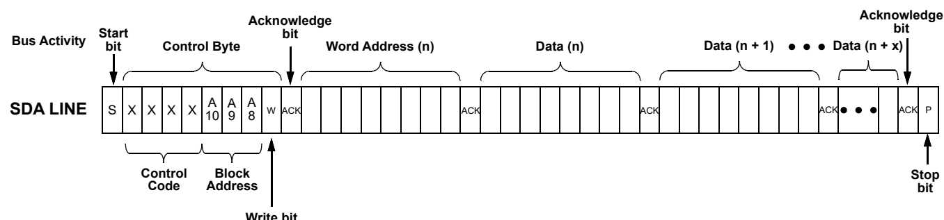
Figure 93: Sequential Write Command
