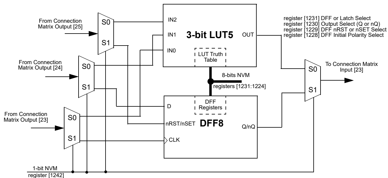
Figure 23: 3-bit LUT5 or DFF8
