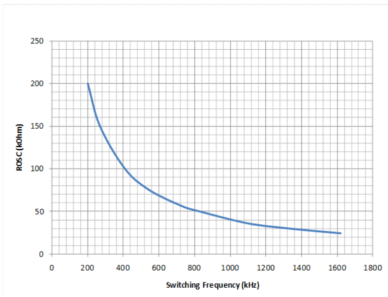
Figure 34. ROSC vs Switching Frequency
