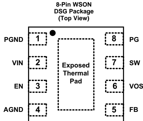
Pin Functions
