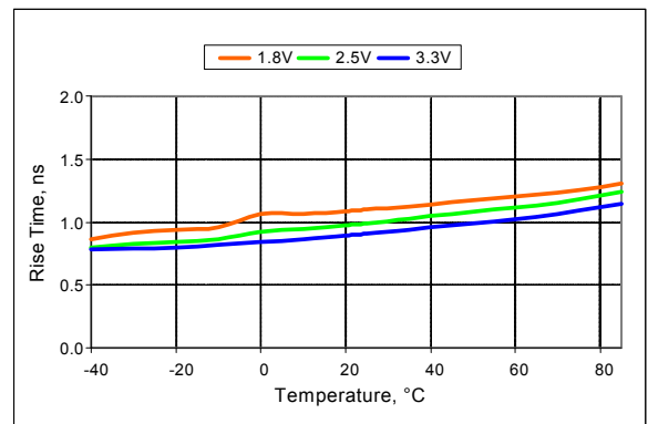
Figure 13. Rise Time vs Temperature, 75 MHz Output
