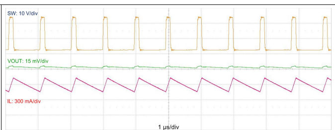
Figure 14. Typical PWM Switching Waveforms V_{IN} = 24\text{ V} , V_{OUT} = 5\text{ V} , I_{OUT} = 600\text{ mA} , f_s = 1000\text{ kHz}
