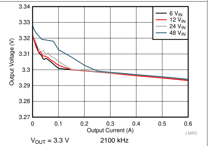
Figure 46. Load Regulation
