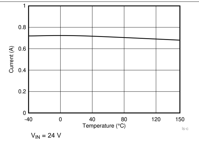
Figure 4. Low Side Current Limit
