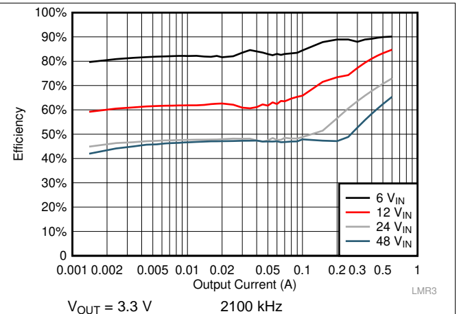
Figure 44. Efficiency
