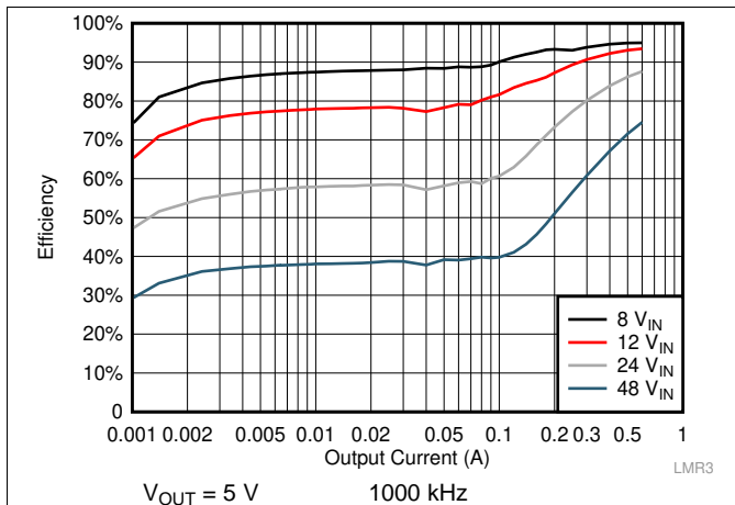
Figure 21. Efficiency
