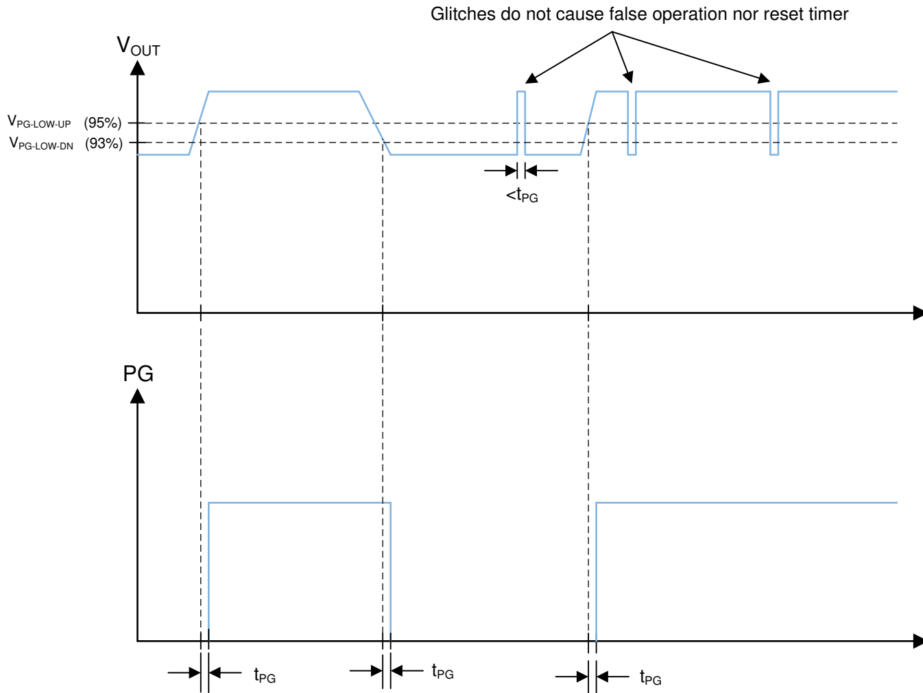
Figure 9. Power-Good-Timing Behavior
