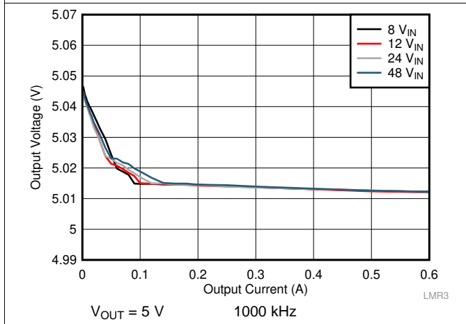
Figure 23. Load Regulation
