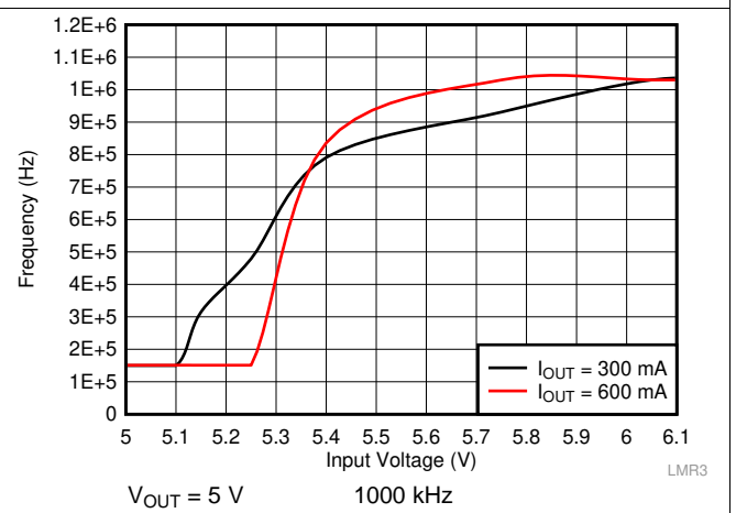
Figure 26. Frequency Dropout Characteristic
