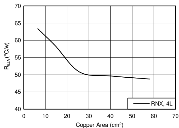
Figure 20. R_{\theta JA} versus Copper Board Area for the VQFN (RNX) Package
