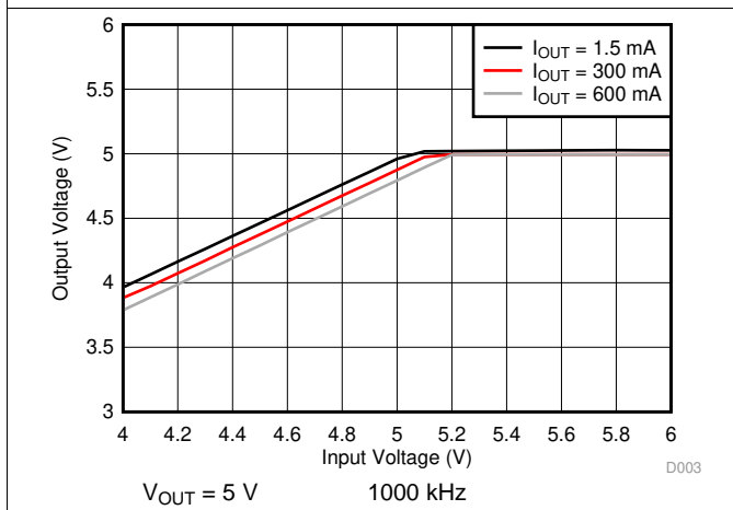
Figure 25. Overall Dropout Characteristic
