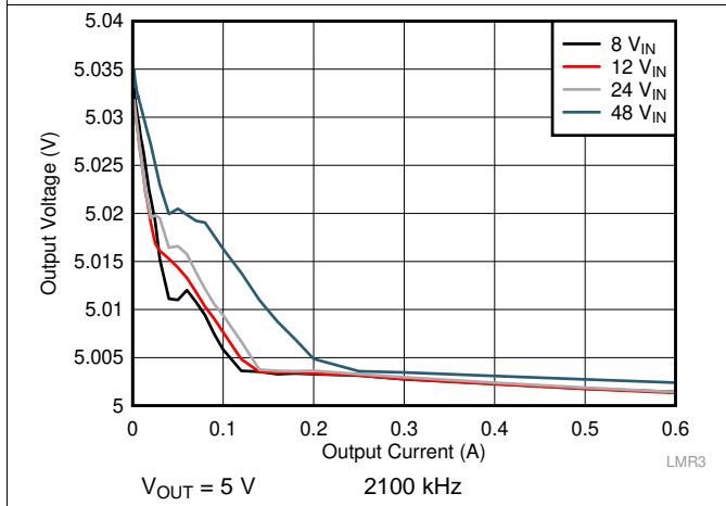
Figure 45. Load Regulation
