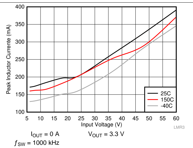
Figure 6. I PEAK-MIN
