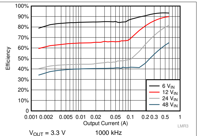
Figure 22. Efficiency
