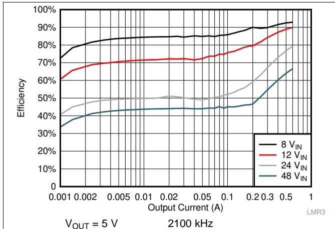
Figure 43. Efficiency
