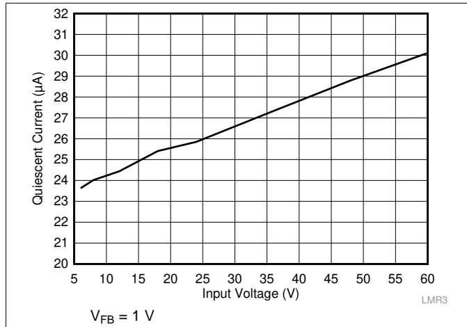
Figure 1. Non-Switching Input Supply Current
