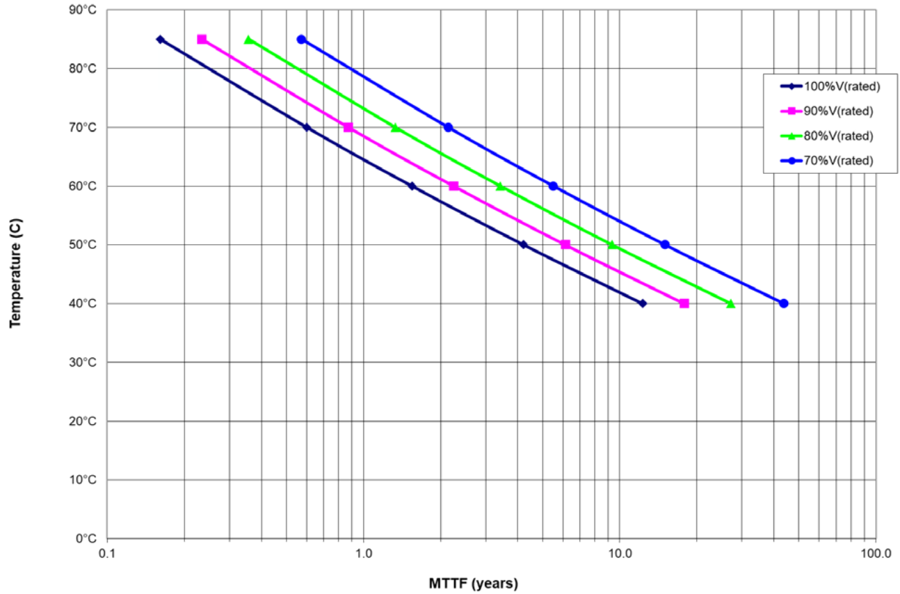
Expected Lifetime at Various Voltages SCC series 2.7V Rated
