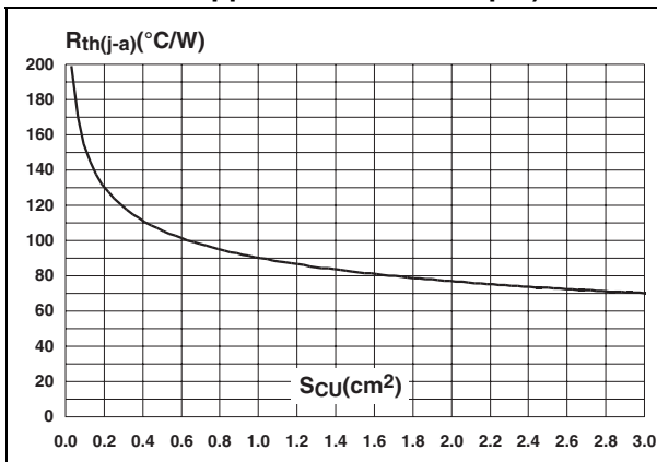
Figure 9. Thermal resistance junction to ambient versus copper surface under each lead (printed circuit board FR4, copper thickness = 35 \mu m)
