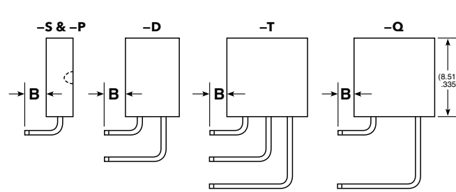
Right-angle Versions
