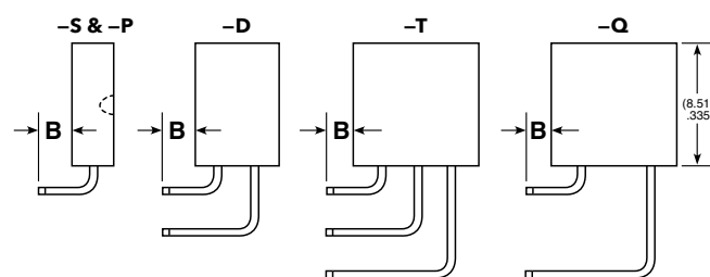
Right-angle Versions
