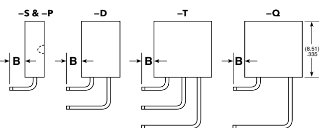
Right-angle Versions
