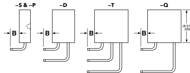
Right-angle Versions
