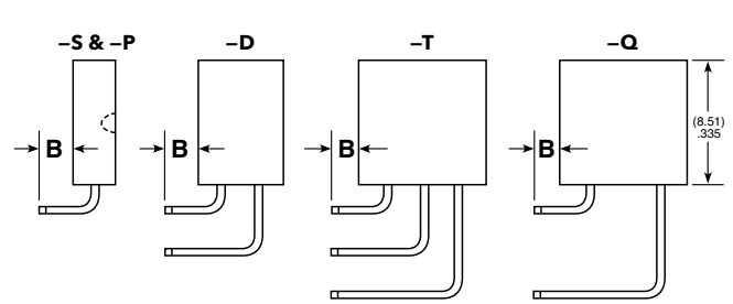
Right-angle Versions
