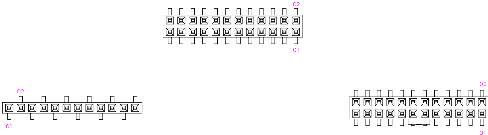
FIG 4 POLARIZATION LOCATION INSERT PK-15-N INTO SPECIFIED POS AND BREAK OFF TAB
