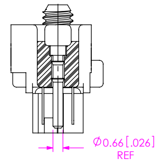
SECTION "F"-"F"
