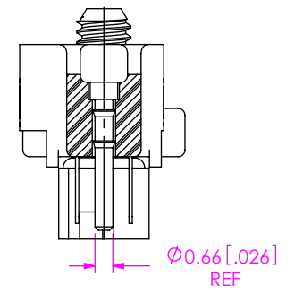
SECTION "F"-"F"
