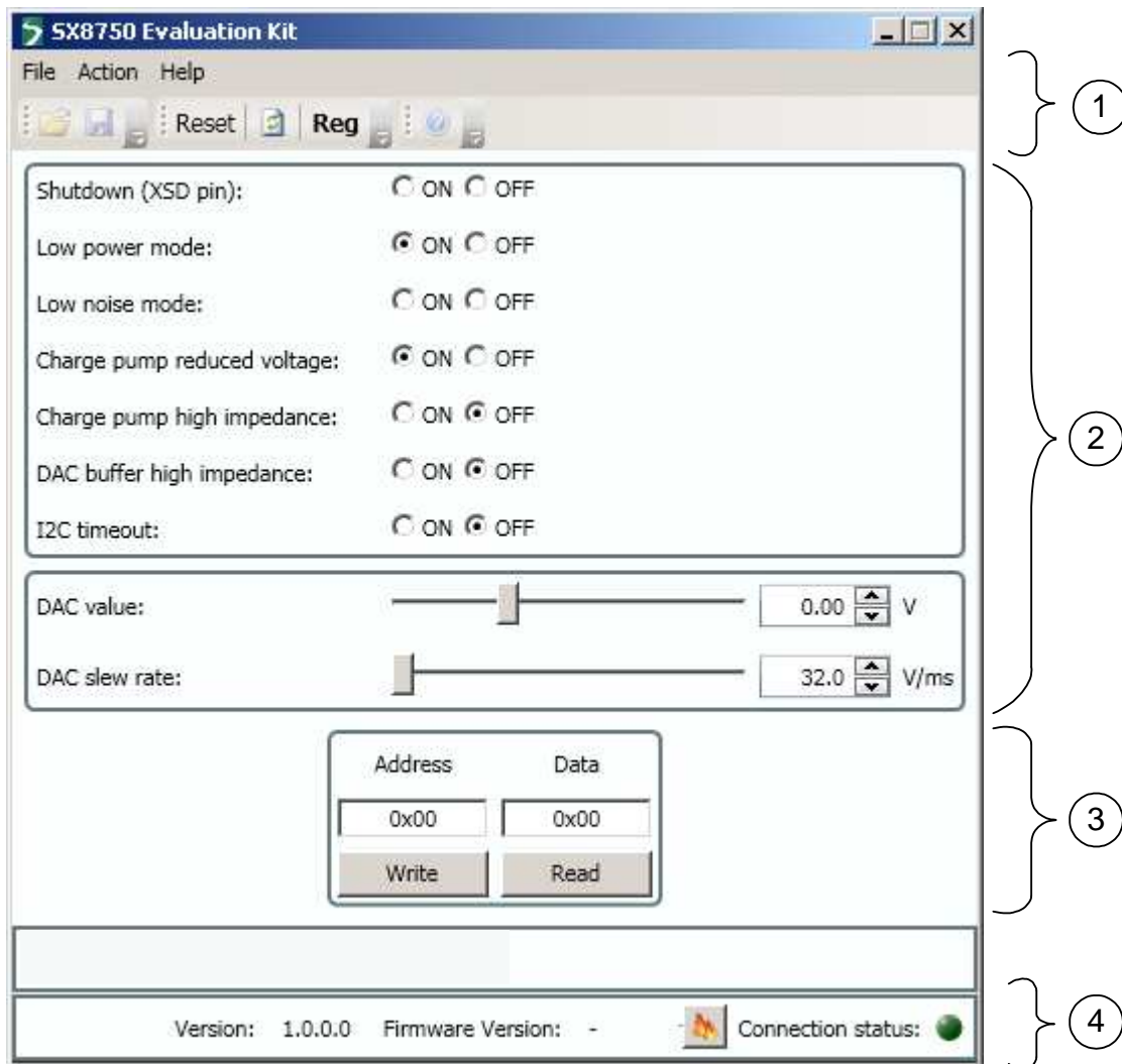
Figure 3. GUI overview
