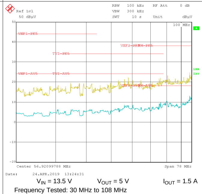
Figure 37. Conducted EMI vs. CISPR25 Limits (Yellow: Peak Signal, Blue: Average Signal)
