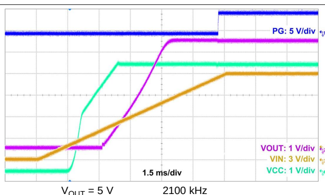
Figure 51. Start-Up Waveform
