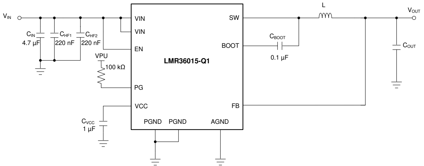
Figure 19. Example Applications Circuit (Fixed 3.3 V Output)
