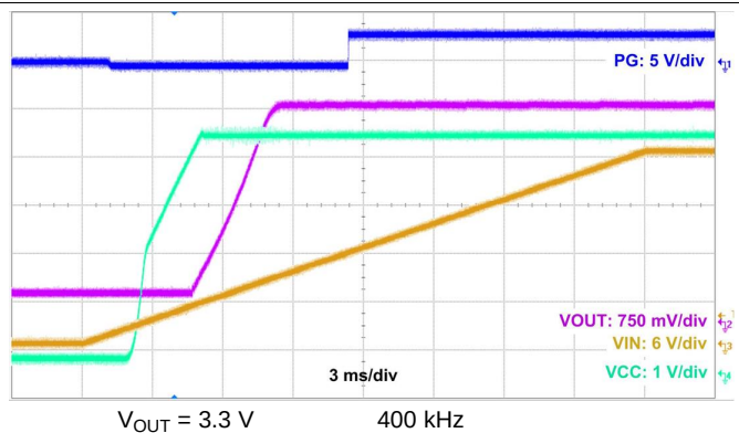
Figure 33. Start-Up Waveform
