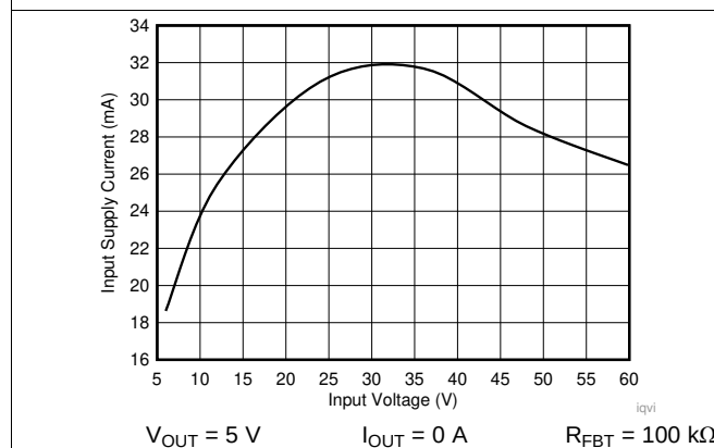
Figure 50. Input Supply Current
