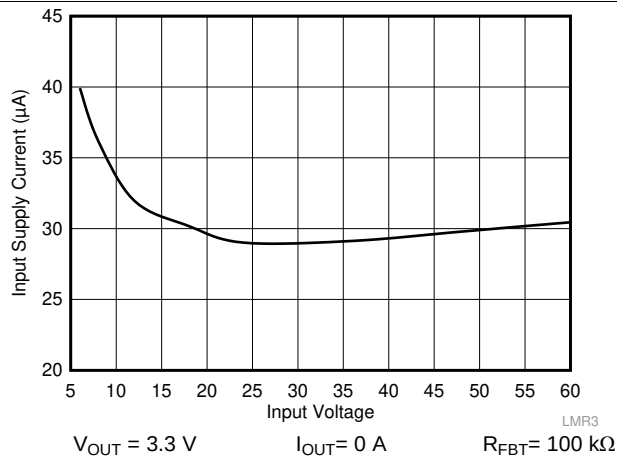
Figure 30. Input Supply Current
