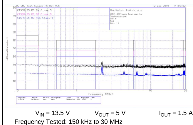
Figure 38. Radiated EMI Rod vs. CISPR25 Limits
