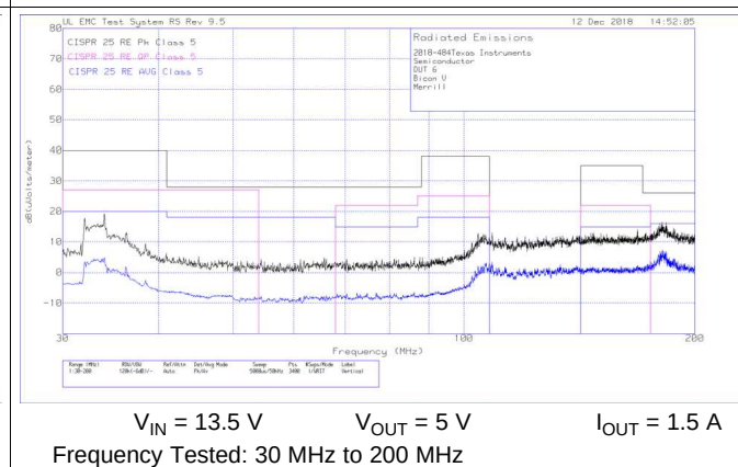
Figure 39. Radiated EMI Bicon Vertical vs. CISPR25 Limits
