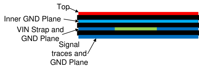
Figure 54. Example Layout
