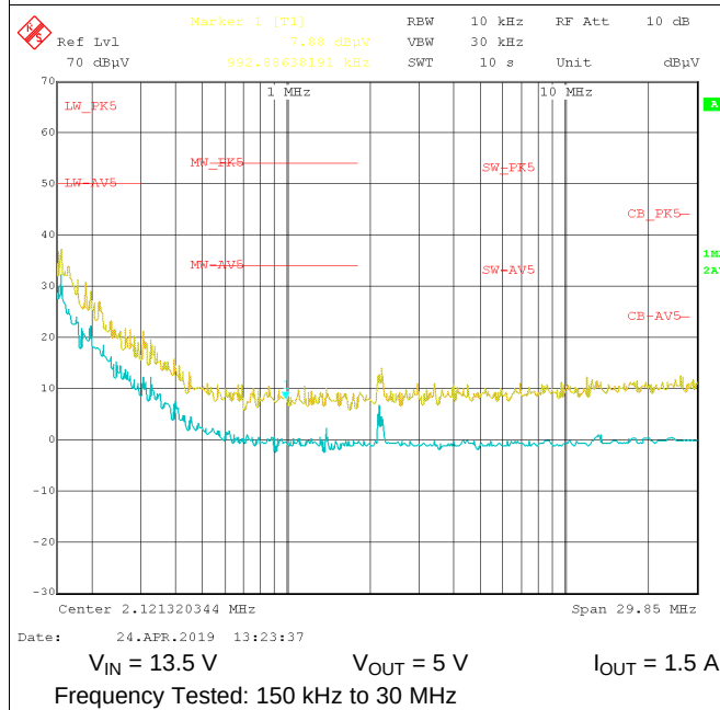
Figure 36. Conducted EMI vs. CISPR25 Limits (Yellow: Peak Signal, Blue: Average Signal)
