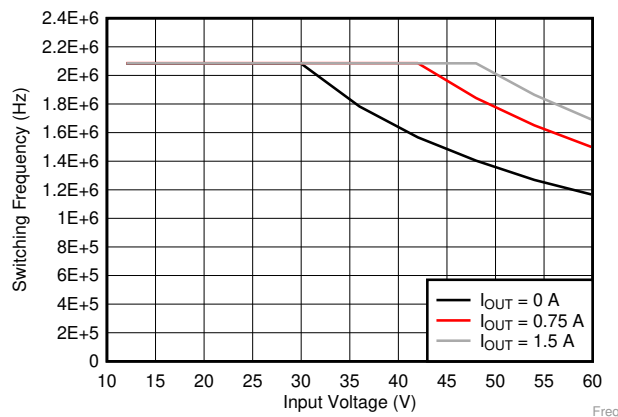
Figure 17. Switching Frequency vs Input Voltage V OUT = 5 V
