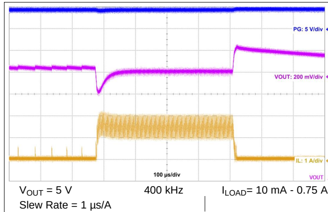
Figure 34. Load Transient
