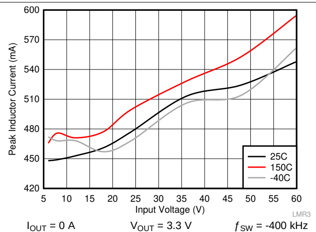
Figure 6. I_{PEAK-MIN}
