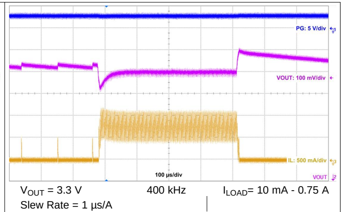
Figure 35. Load Transient
