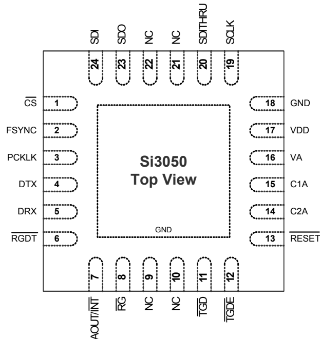
Figure 50. Si3050 QFN
