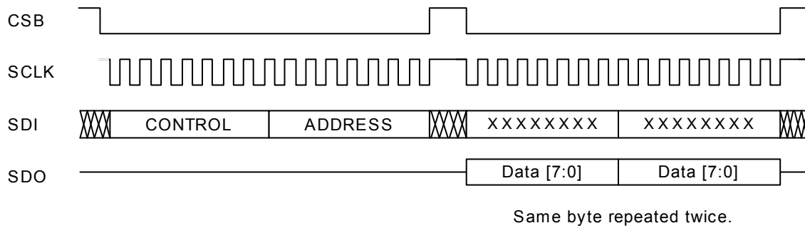
Figure 42. Read Operation via a 16-bit SPI Port
