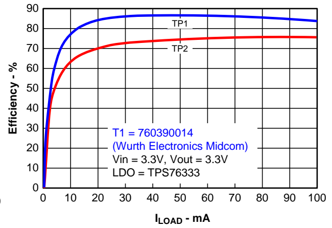
Figure 15. Efficiency Versus Load Current V_{in} = 3.3\text{ V} , V_{out} = 3.3\text{ V}
