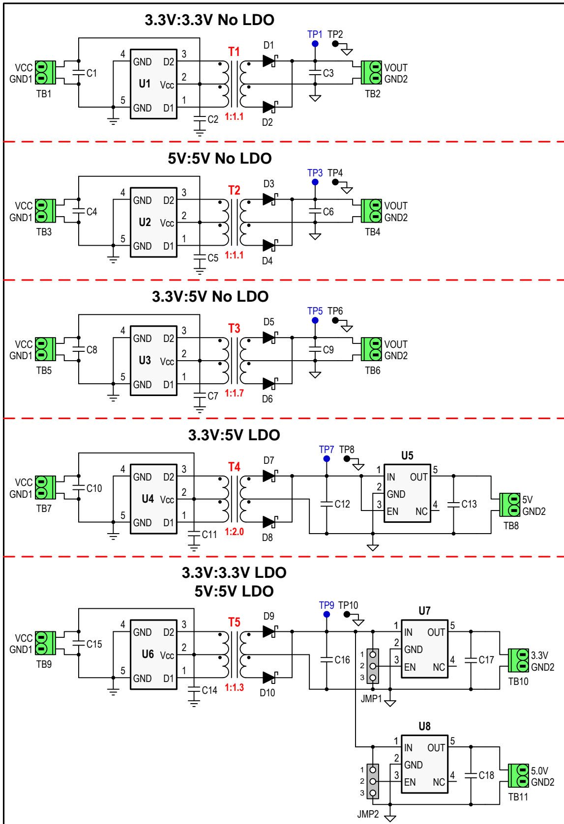
Figure 3. SN6501 EVM Schematic
