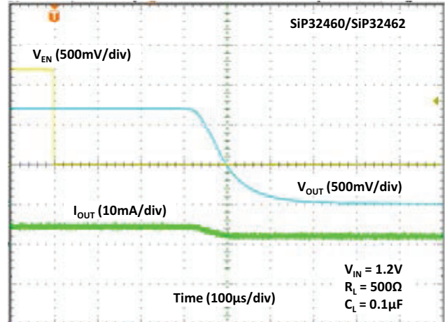
Fig. 35 - Turn-off Time
