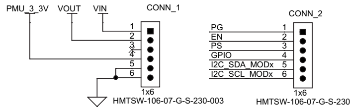
SUB-MODULE CONNECTORS
