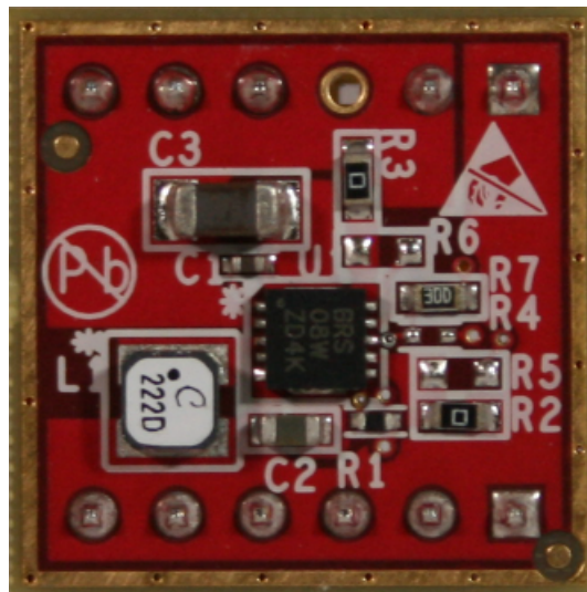
Figure 1. SMP-TPS61201-MVK Submodule
