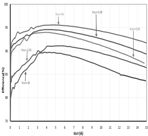
Efficiency Variation with V_{OUT} - P-Save ( V_{DD} = 5\text{ V} , V_{IN} = 12\text{ V} , L = 22\text{ }\mu\text{H} (4.6 m \Omega )) for V_{OUT} = 2.5\text{ V} , 3.3\text{ V} and 5\text{ V} , SiC401B)
