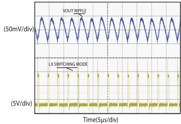
Forced Continuous Mode (V DD = 5 V, V IN = 12 V, V OUT = 1.5 V, I OUT = 15 A, SiC401B)
