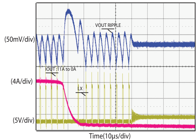
Transient Response - P-Save Load Falling (V DD = 5 V, V IN = 12 V, V OUT = 1.5 V, I OUT = 11 A to 0 A, SiC401B, dl/dt = 1 A/µs)
