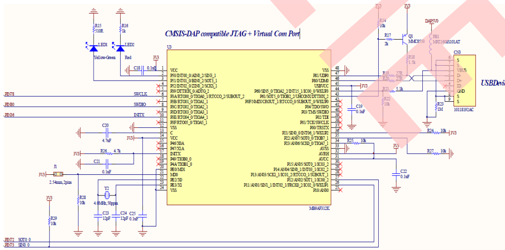
Figure 21. CMSIS-DAP Compatible JTAG + Virtual Com Port Circuit
