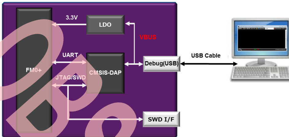
Figure 20. CMSIS-DAP Block
