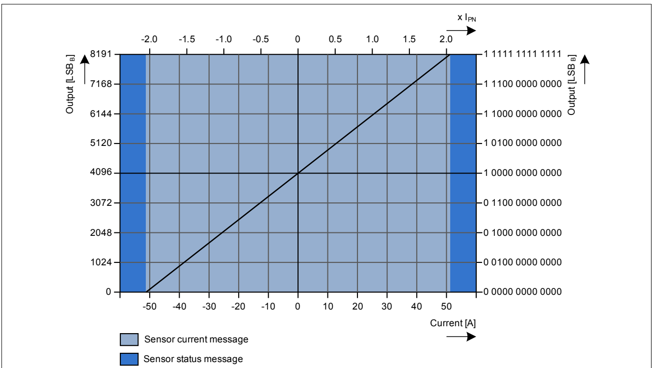
Figure 2-4 Transfer function
