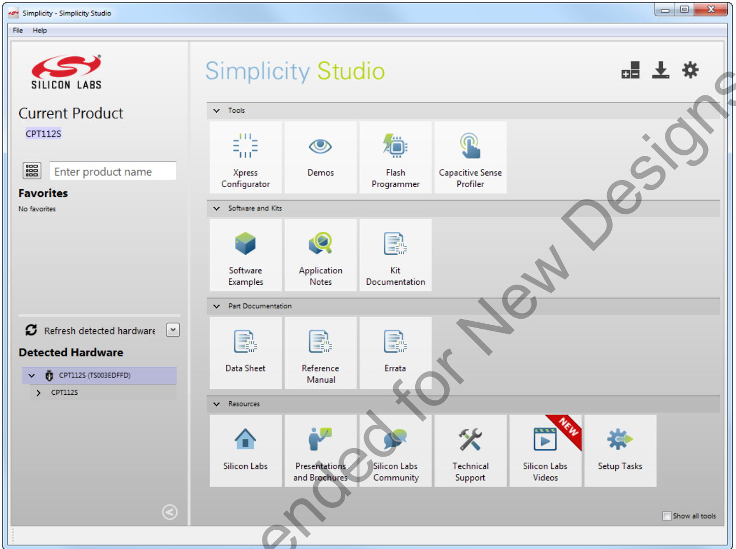
Figure 7.1. Simplicity Studio
