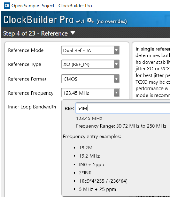
Figure 51. Correcting the Reference Frequency
