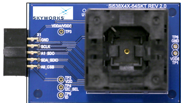
Figure 8. Si538x4x-64SKT-DK
