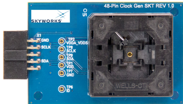
Figure 6. Si5332-48SKT-DK
