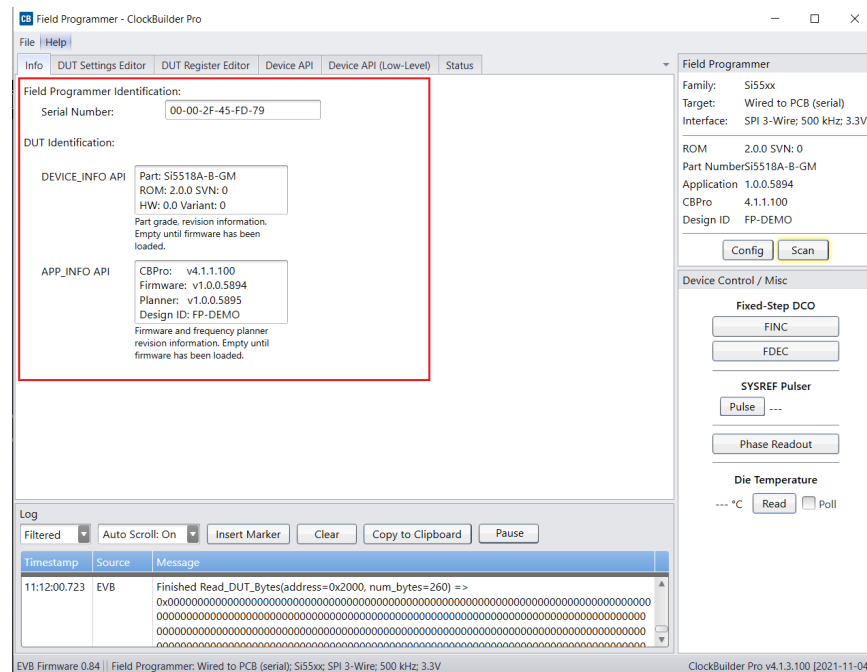
Figure 49. Device info is Displayed after a Successful Scan Operation (Si5518 Device)
