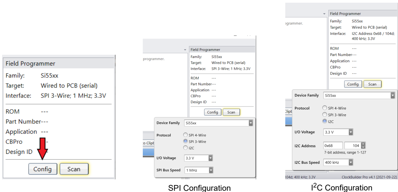
Figure 48. Configuring an In-System Device
