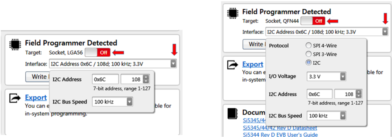
Figure 42. Interface Settings
