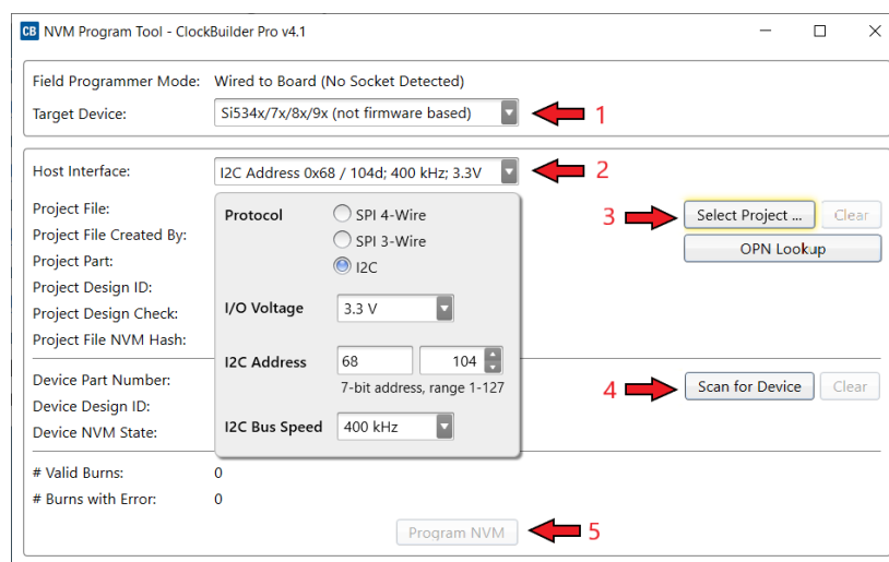
Figure 31. Programming In-system, Non-firmware Based Devices
