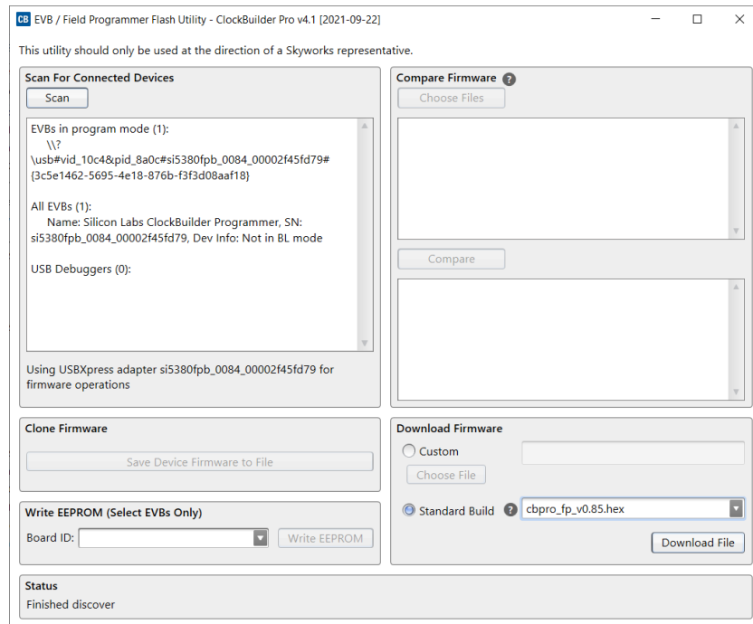
Figure 61. Select the Latest Field Programmer Firmware Image
