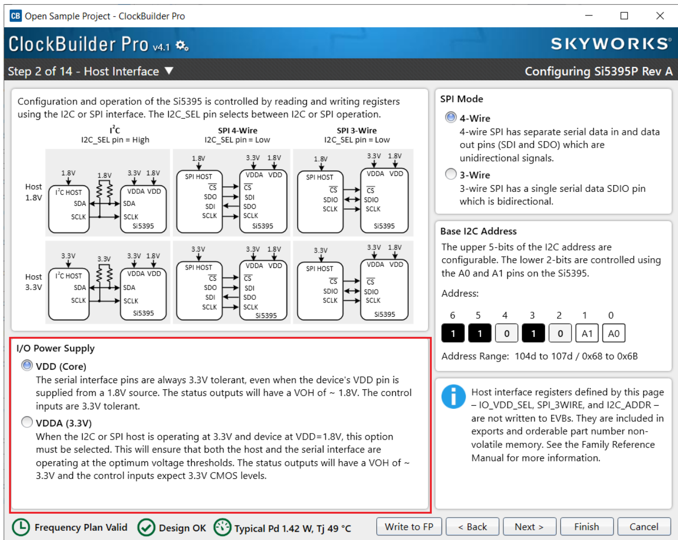
Figure 73. Determine the Value of IO_VDD_SEL Bit Written to Device
