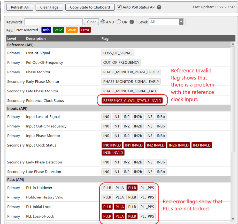
Figure 50. EVB GUI Reference Error Example, Si5518
