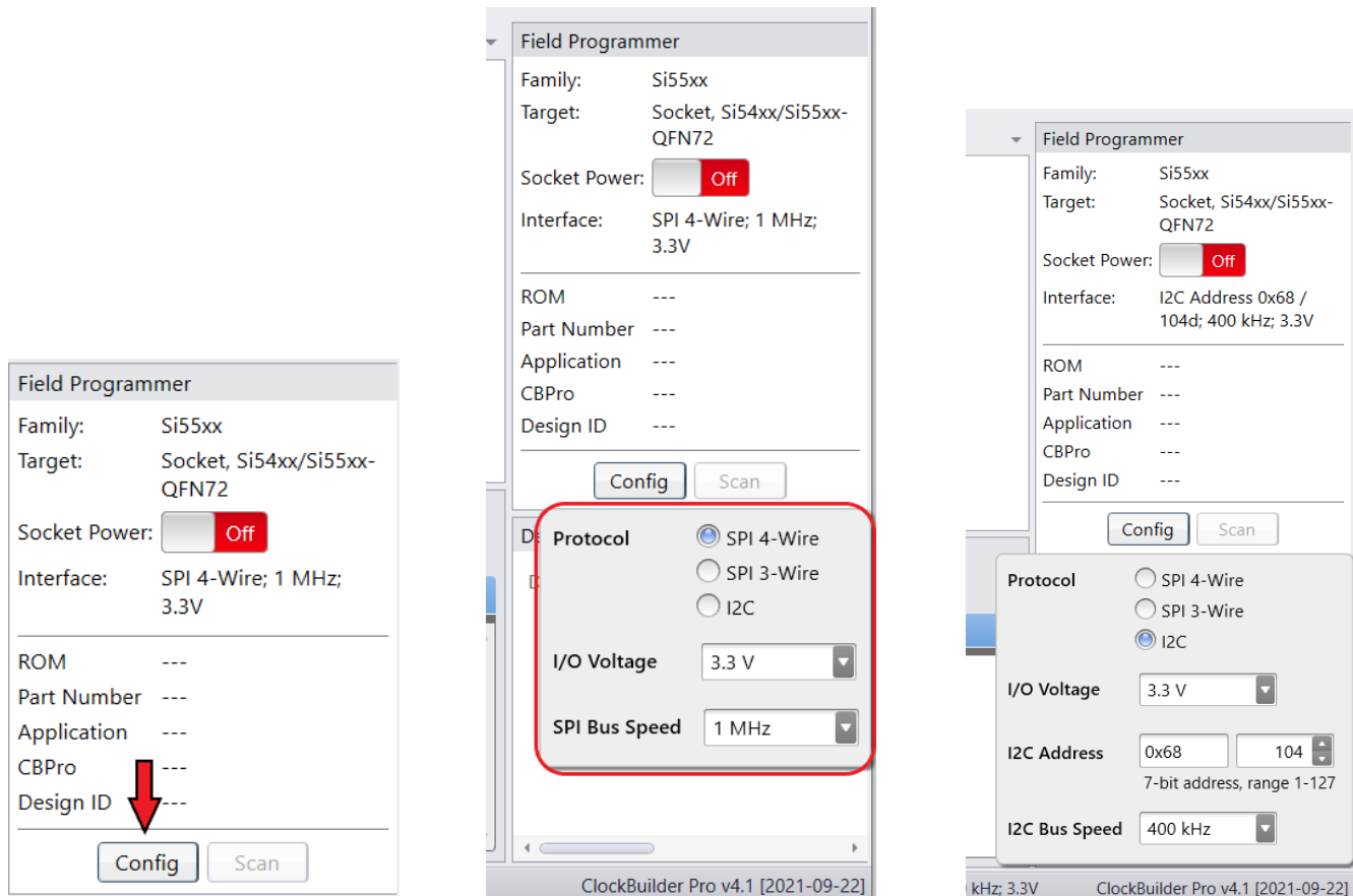
SPI Devices Configuration
