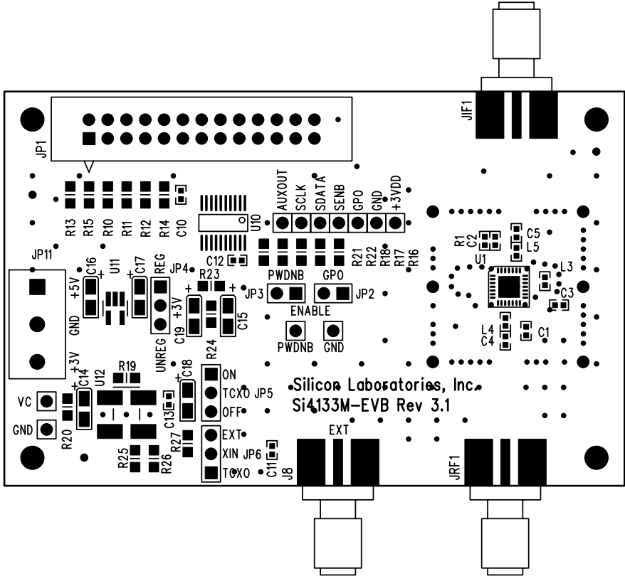
Figure 28. Si4133M Silkscreen
