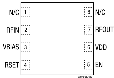
Figure 2. SKY67189-396LF Pinout (Top View)
