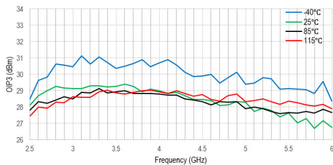
Figure 8. OIP3 (dBm) vs Frequency (GHz)
