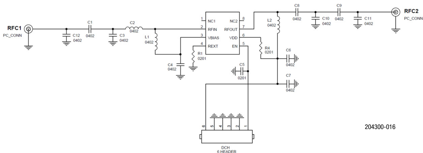
Figure 16. SKY67189-396LF Evaluation Board Schematic for 2500 to 6000 MHz Tuning
