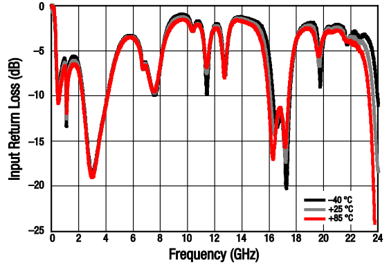
Figure 22. Input Return Loss vs Frequency (Wide Band) Over Temperature
