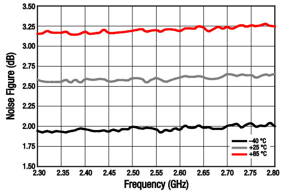
Figure 13. Noise Figure vs Frequency Over Temperature (Includes EVB Losses)
