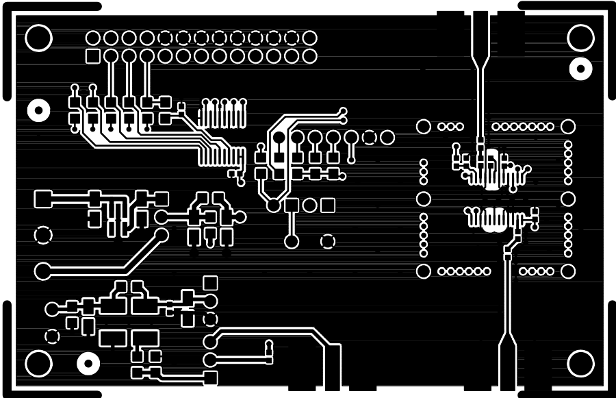
Figure 49. Si4136BT Component
