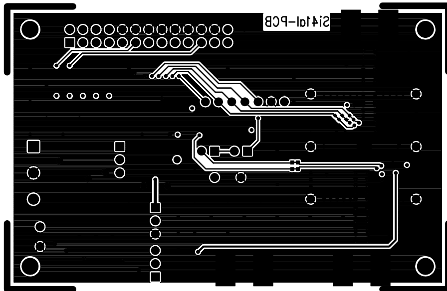
Figure 32. Si4133M Solder
