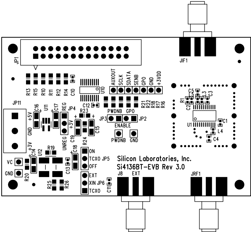
Figure 48. Si4136BT Silkscreen
