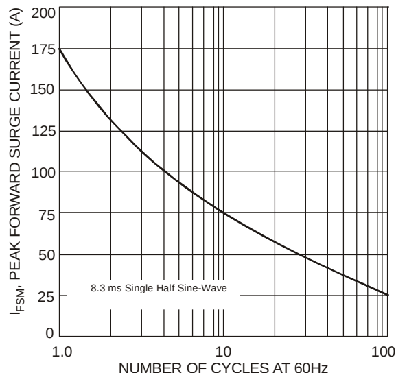
Fig. 4 Max Non-Repetitive Peak Fwd Surge Current
