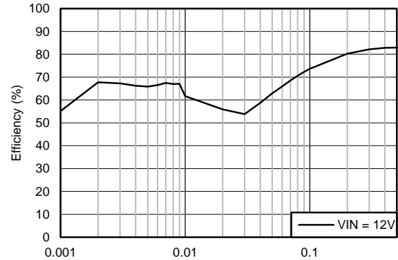
Figure 78. Efficiency
