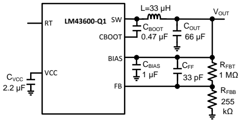
Figure 59. BOM for V_{OUT} = 5\text{ V} F_S = 500\text{ kHz}
