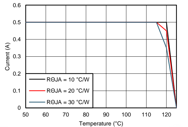
Figure 58. Derating Curve
