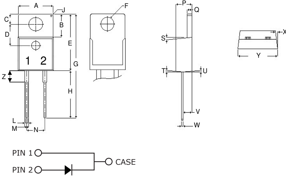
Package TO-220-2
