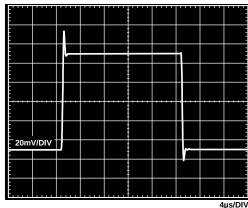
Figure 43. Small Signal Pulse Response, G = 1 , R_{LOAD} = 2\text{ k}\Omega , C_{LOAD} = 100\text{ pF} , V_S = \pm 15\text{ V} , V_{REF} = 0\text{ V}
