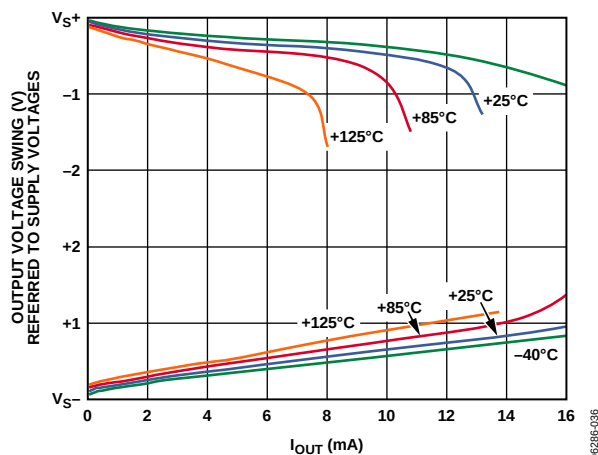
Figure 35. Output Voltage Swing vs. Output Current, V_S = 5\text{ V} , V_{REF} = 2.5\text{ V}
