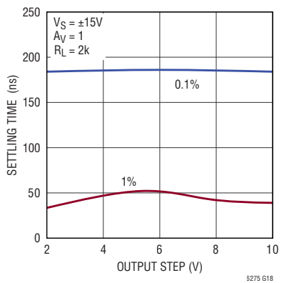
Settling Time vs Output Step
