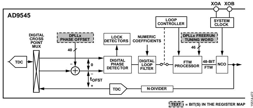
Figure 80. DPLL Phase Offset Feature
