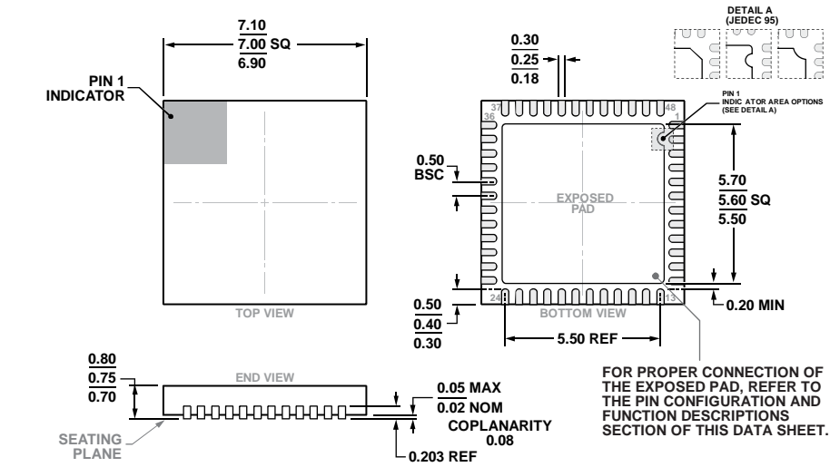
COMPLIANT TO JEDEC STANDARDS MO-220-WKKD-4. Figure 134. 48-Lead Lead Frame Chip Scale Package [LFCSP] 7 mm × 7 mm Body and 0.75 mm Package Height (CP-48-13) Dimensions shown in millimeters
