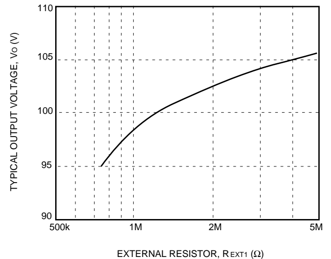
Figure 4. External Resistor Values for Output Voltages from 95 V to 110 V
