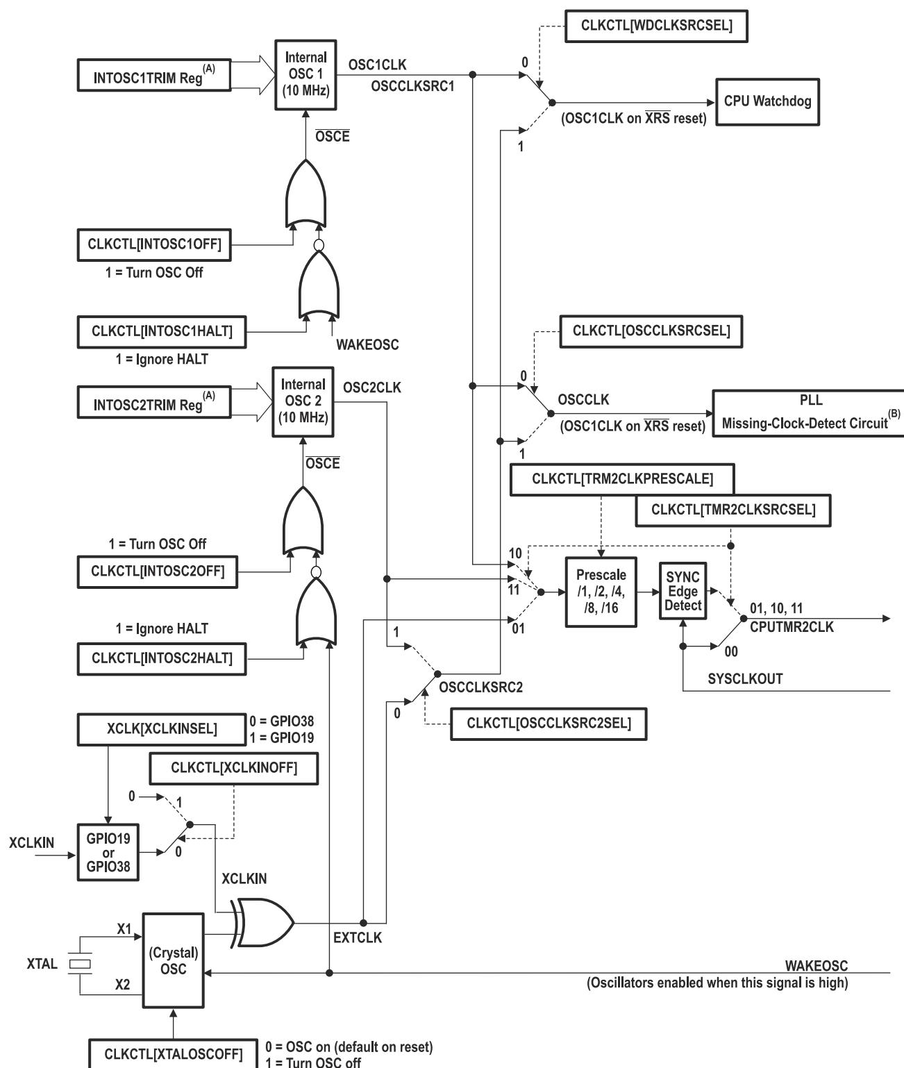
Figure 9-8. Clock Tree
