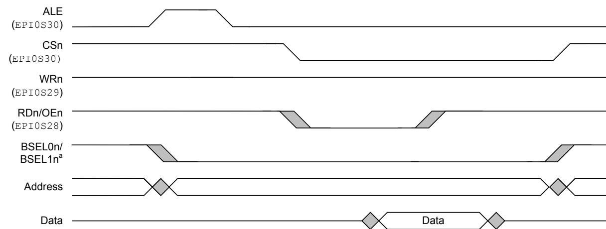
Figure 10-5. Host-Bus Read Cycle, MODE = 0x1, WRHIGH = 1, RDHIGH = 1
