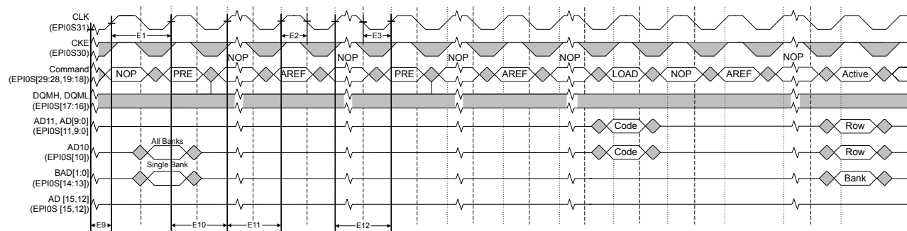
Figure 27-10. SDRAM Initialization and Load Mode Register Timing
