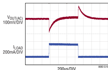
Transient Response from 24V_{IN} to 12V_{OUT}
