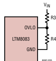
Figure 5. V IN Overvoltage Lockout (OVLO)
