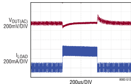
Transient Response from 36V_{IN} to 5V_{OUT}
