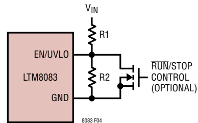
Figure 4. V IN Undervoltage Lockout (UVLO)
