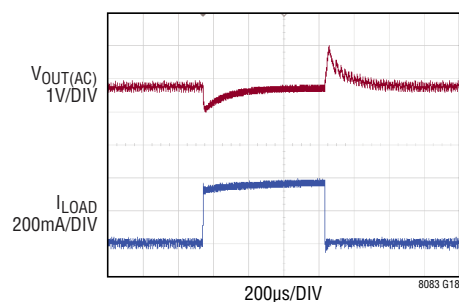
Transient Response from 36V_{IN} to 36V_{OUT}
