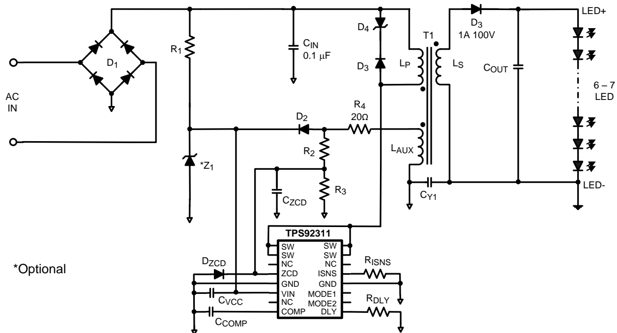
Figure 1. Typical Application
