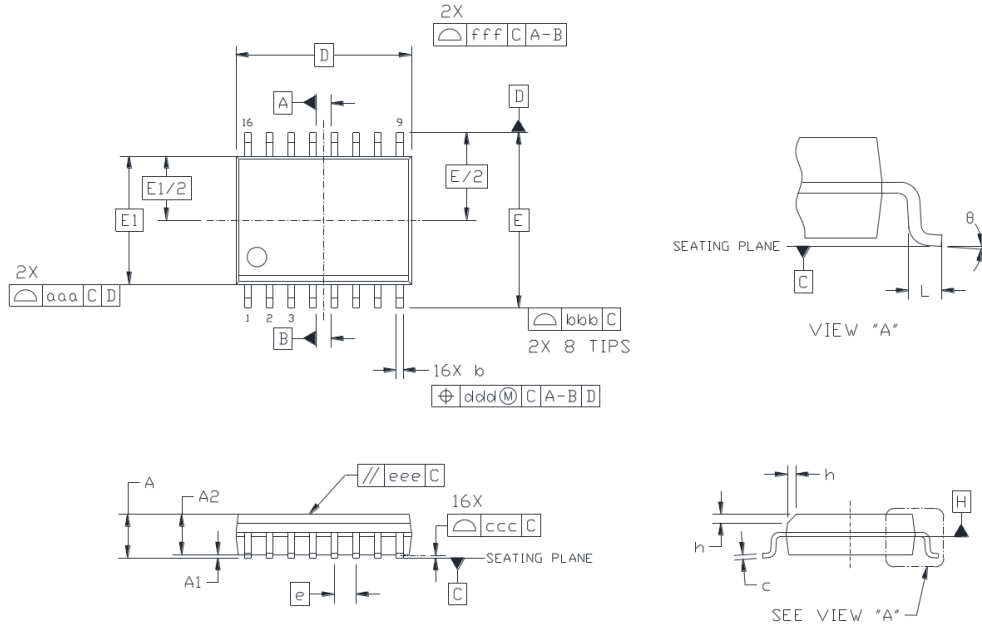
Figure 16. WB SOIC-16
