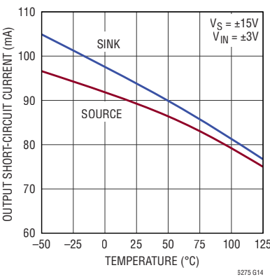
Output Short-Circuit Current vs Temperature
