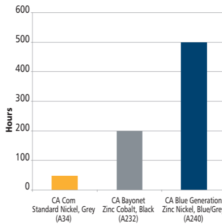
Salt spray resistance with RoHS compliant platings
