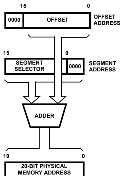
FIGURE 6. 80C286 REAL ADDRESS MODE ADDRESS CALCULATION
