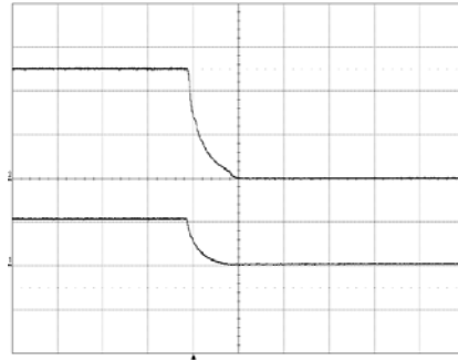
Shut-down enabled by disconnecting V_I at: T_{ref} = +25^{\circ}\text{C} , V_I = 53\text{ V} , I_O = 38\text{ A} resistive load.
