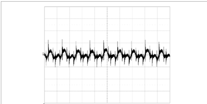
Output voltage ripple at: T_{ref} = +25^{\circ}C , V_1 = 53 V , I_o = 40 A resistive load.
