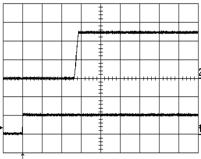
Start-up enabled by connecting V_I at: T_{ref} = +25^{\circ}\text{C} , V_I = 53\text{ V} , I_O = 38\text{ A} resistive load.
