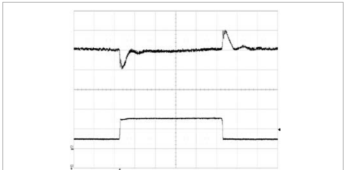
Output voltage response to load current step- change (10 - 30 - 10 A) at: T_{ref} = +25^{\circ}C , V_1 = 53 V , C_o = 4 mF
