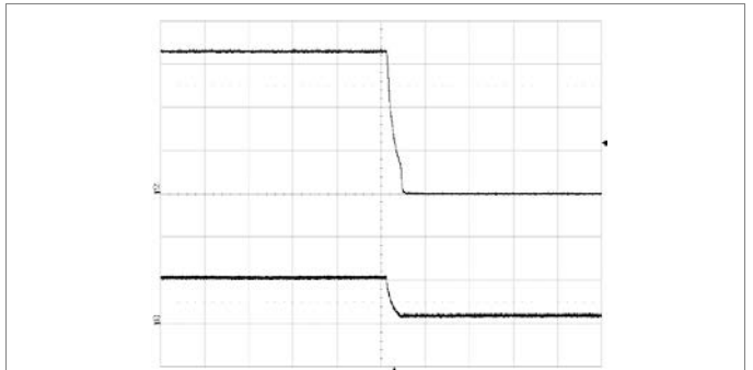
Shut-down enabled by disconnecting V_1 at: T_{ref} = +25^{\circ}C , V_1 = 53 V , I_o = 40 A resistive load.
