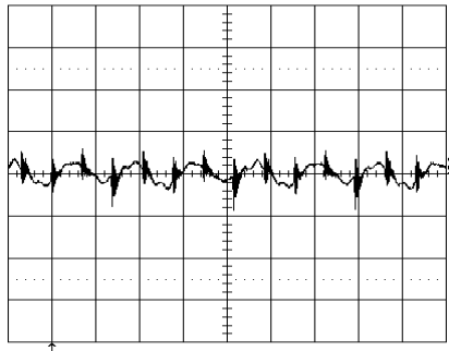
Output voltage ripple at: T_{ref} = +25^{\circ}\text{C} , V_I = 53\text{ V} , I_O = 38\text{ A} resistive load.
