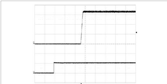
Start-up enabled by connecting V_1 at: T_{ref} = +25^{\circ}C , V_1 = 53 V , I_o = 40 A resistive load.
