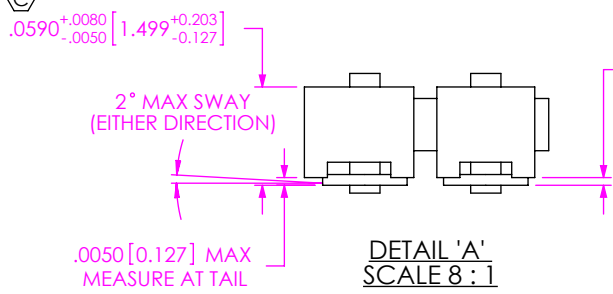
FIG 4 -MW: METAL WASHER OPTION MTMM-1XX-02-XX-X-100-MW SHOWN (ONE PER POSITION) (-D & -Q BODY SPEC ONLY, SEE NOTE 5) (SAME AS FIG 1, DIFFERENT AS SHOWN) ** -MW OPTION, DO NOT DESIGN IN. SAMTEC WILL ONLY SUPPORT EXISTING BUSINESS 02/08/2002
