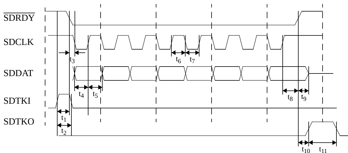
Figure 6. SD Port Read Timing
