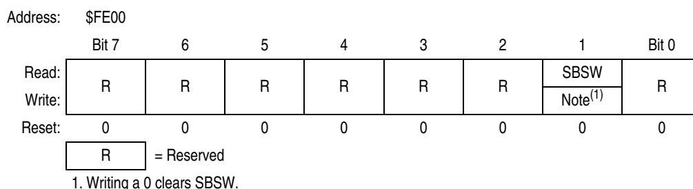
Figure 15-20. Break Status Register (SBSR)
