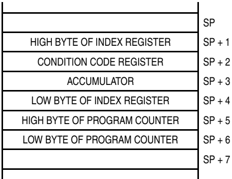
Figure 19-16. Stack Pointer at Monitor Mode Entry
